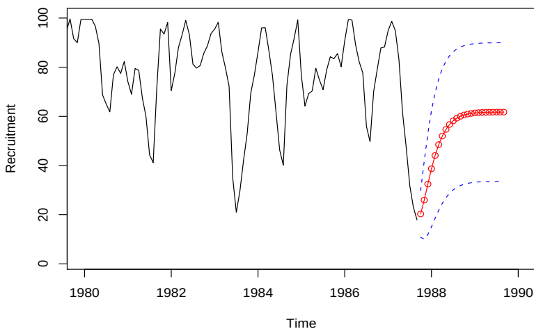
Fig. 3.7. Twenty-four month forecasts for the Recruitment series. The actual data shown are from about January 1980 to September 1987, and then the forecasts plus and minus one standard error are displayed.
