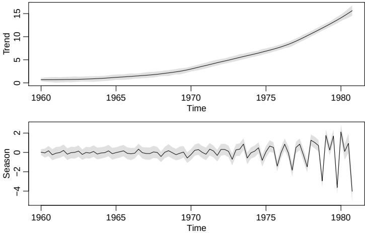
Fig. 6.19. Example 6.23 smoother estimates of trend ( T_t ) and season ( S_t ) along with corresponding 99% credible intervals.
