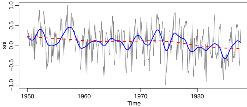
Fig. 2.15. Smoothing splines fit to the SOI series.
