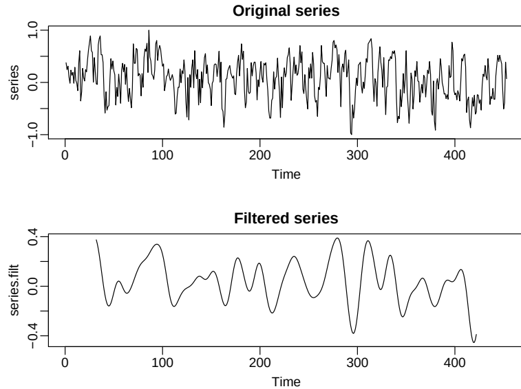
Fig. 4.20. Original SOI series (top) compared to filtered version showing the estimated El Niño temperature signal (bottom).
