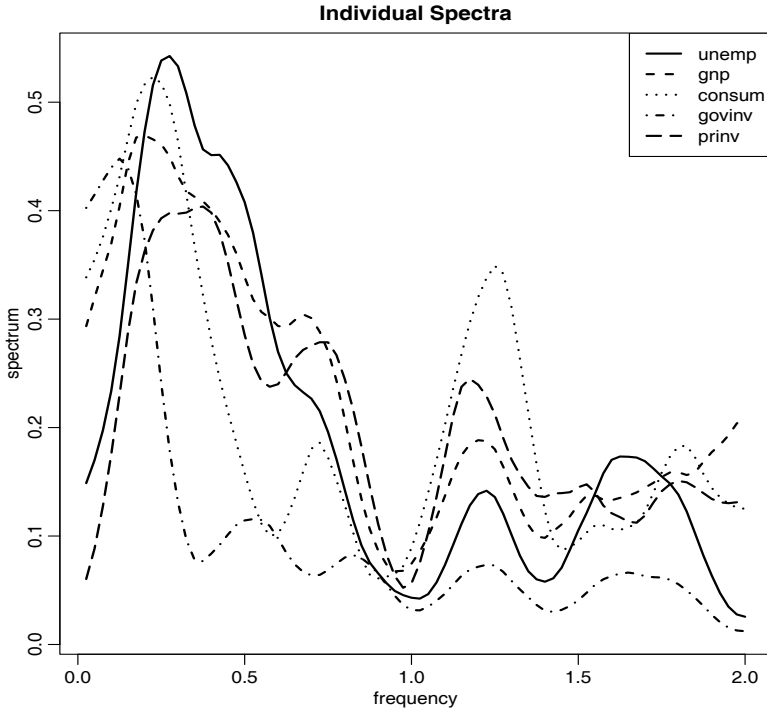
Fig. 7.20. The individual estimated spectra (scaled by 1000) of each series show in Figure 7.19 in terms of the number of cycles in 160 quarters.
