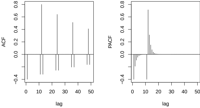
Fig. 3.24. ACF and PACF of the mixed seasonal ARMA model x_t = .8x_{t-12} + w_t - .5w_{t-1} .
