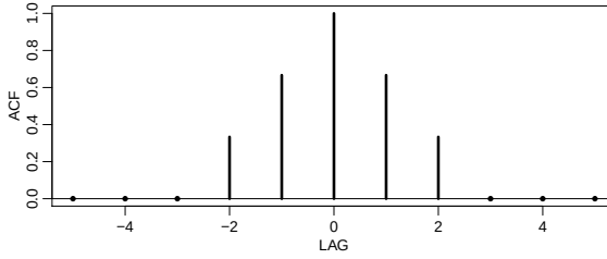
Fig. 1.12. Autocorrelation function of a three-point moving average.
