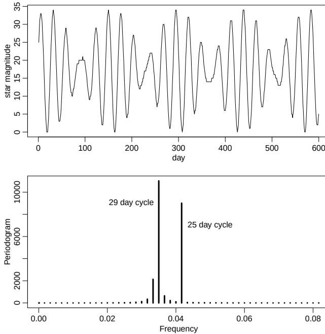
Fig. 4.3. Star magnitudes and part of the corresponding periodogram.
