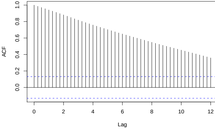
Fig. 3.15. Sample ACF of the GNP data. Lag is in terms of years.
