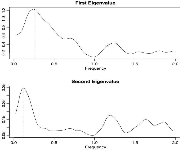
Fig. 7.22. The first, \hat{\lambda}_1(\omega) , and second, \hat{\lambda}_2(\omega) , eigenvalues of the estimated spectral matrix \hat{f}_{xx}(\omega) . The vertical dashed lines are shown at \omega = .25 and .125 , respectively.
