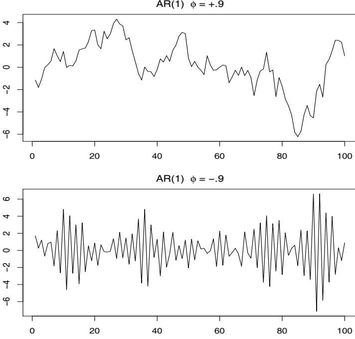
Fig. 3.1. Simulated AR(1) models: \phi = .9 (top); \phi = -.9 (bottom).
