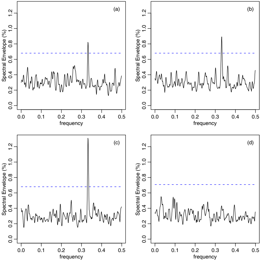
Fig. 7.25. Smoothed sample spectral envelope of the BNRF1 gene from the Epstein–Barr virus: (a) first 1000 bp, (b) second 1000 bp, (c) third 1000 bp, and (d) last 954 bp.
