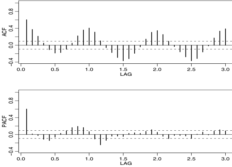
Fig. 5.9. Sample ACF and PACF of SOI.
