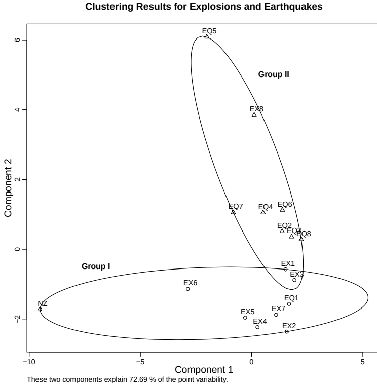
Fig. 7.16. Clustering results for the earthquake and explosion series based on symmetric divergence using a robust version of k-means clustering with two groups. Circles indicate Group I classification, triangles indicate Group II classification.
