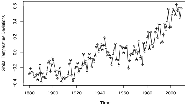
Fig. 1.2. Yearly average global temperature deviations (1880–2009) in degrees centigrade.
