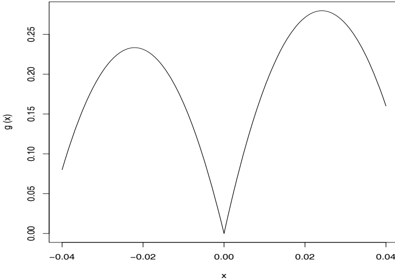
Fig. 7.27. Estimated optimal transformation, (7.187), for the GNP residuals at \omega = .018 .
