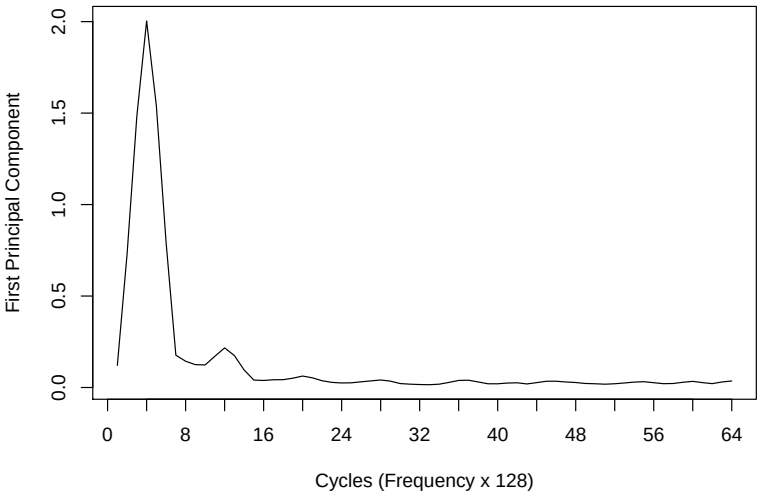
Fig. 7.18. The estimated spectral density, \hat{\lambda}_1(j/128) , of the first principal component series in Example 7.14.
