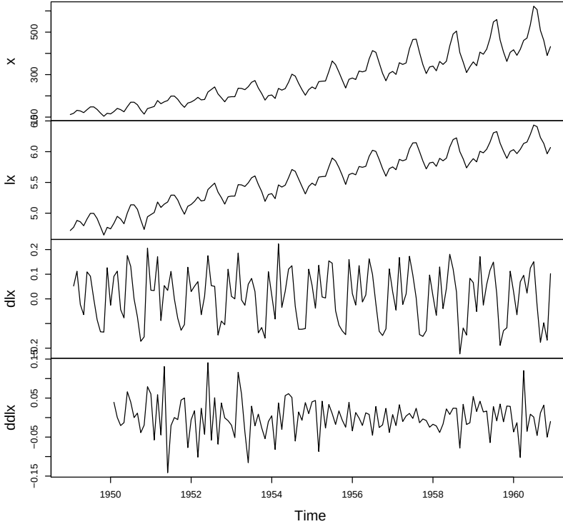
Fig. 3.25. R data set AirPassengers , which are the monthly totals of international airline passengers x , and the transformed data: lx = \log x_t , dlx = \nabla \log x_t , and ddlx = \nabla_{12} \nabla \log x_t .
