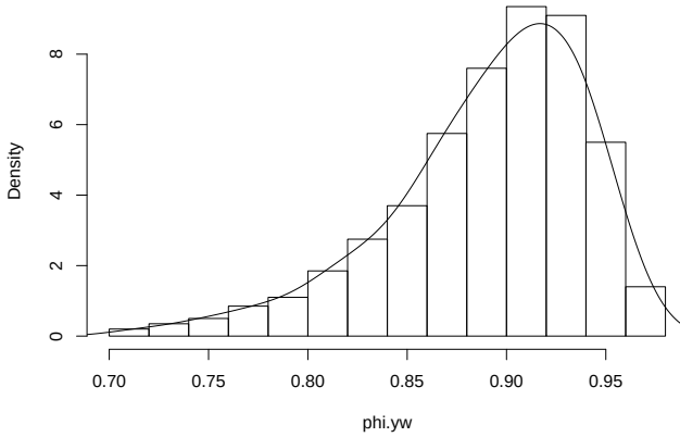
Fig. 3.12. Finite sample density of the Yule-Walker estimate of \phi in Example 3.35 .
