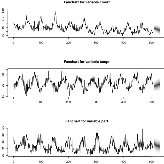
Fig. 5.13. Predictions from a VAR(2) fit to the LA mortality – pollution data.
