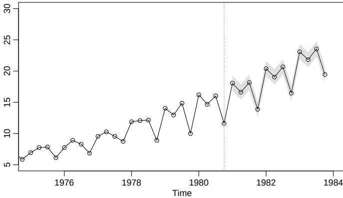
Fig. 6.8. A 12-quarter forecast for the Johnson & Johnson quarterly earnings series. The forecasts are shown as a continuation of the data (points connected by a solid line). The gray area represents three root MSPE bounds.
