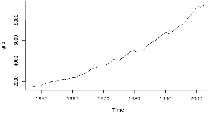
Fig. 3.14. Quarterly U.S. GNP from 1947(1) to 2002(3).
