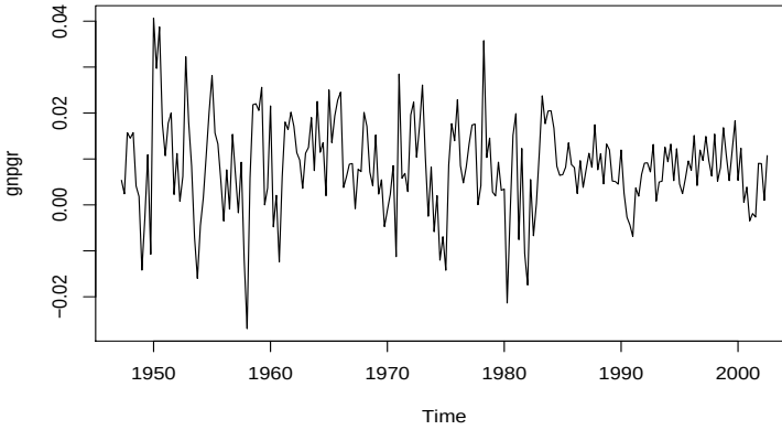
Fig. 3.17. U.S. GNP quarterly growth rate.
