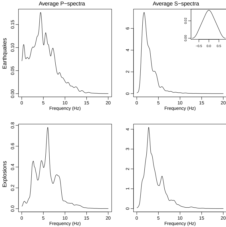
Fig. 7.14. Average P-spectra and S-spectra of the earthquake and explosion series. The insert on the upper right shows the smoothing kernel used; the resulting bandwidth is about .75 Hz.
