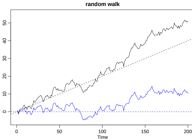
Fig. 1.10. Random walk, \sigma_w = 1 , with drift \delta = .2 (upper jagged line), without drift, \delta = 0 (lower jagged blue line), and straight (dashed) lines with slope \delta .
