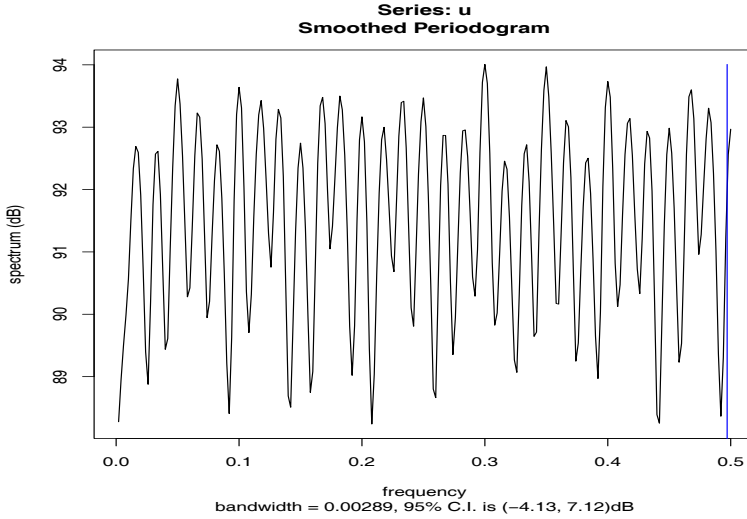
Fig. 7.28. Periodogram, in decibels, of the data generated from (7.188) after tapering by a cosine bell.
