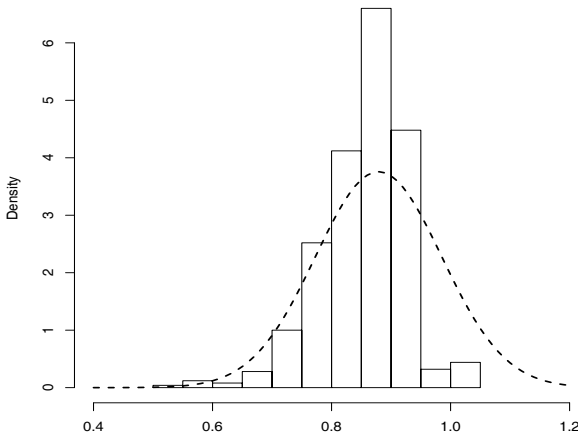
Fig. 6.15. Bootstrap histogram and asymptotic distribution of \hat{\phi}_1 for the U.S. GNP example.
