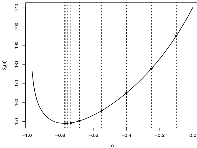
Fig. 3.10. Conditional sum of squares versus values of the moving average parameter for the glacial varve example, Example 3.32 . Vertical lines indicate the values of the parameter obtained via Gauss–Newton; see Table 3.2 for the actual values.
