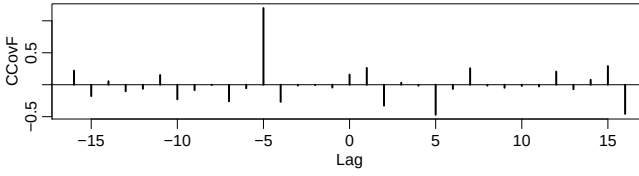
Fig. 1.13. Demonstration of the results of Example 1.23 when \ell = 5 .
