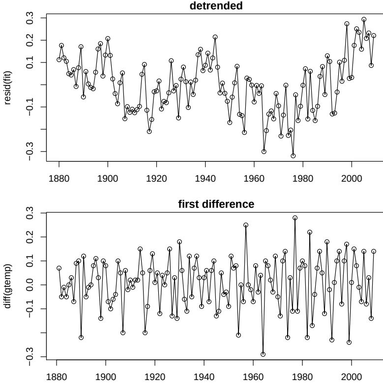
Fig. 2.4. Detrended (top) and differenced (bottom) global temperature series. The original data are shown in Figure 1.2 and Figure 2.1 .
