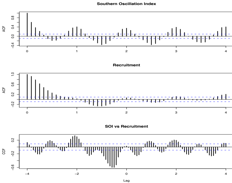
Fig. 1.15. Sample ACFs of the SOI series (top) and of the Recruitment series (middle), and the sample CCF of the two series (bottom); negative lags indicate SOI leads Recruitment. The lag axes are in terms of seasons (12 months).
