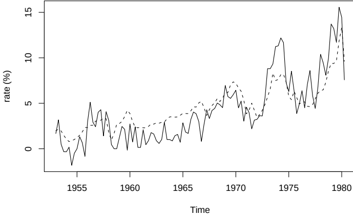
Fig. 6.9. Quarterly interest rate for Treasury bills (dashed line) and quarterly inflation rate (solid line) in the Consumer Price Index.
