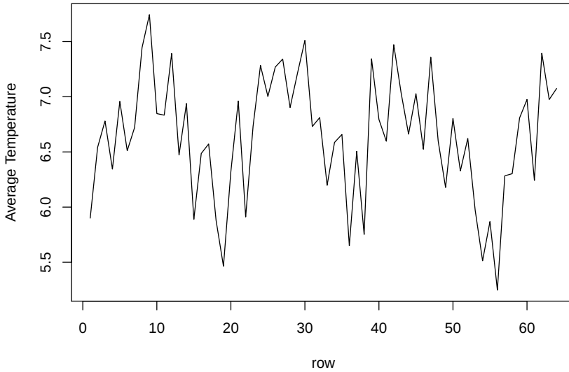
Fig. 1.18. Row averages of the two-dimensional soil temperature profile. \bar{x}_{s_1} = \sum_{s_2} x_{s_1, s_2} / 36 .
