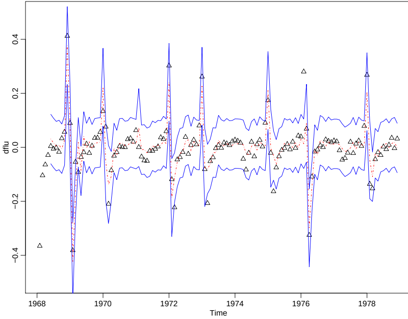
Fig. 5.8. First differenced U.S. monthly pneumonia and influenza deaths (triangles); one-month-ahead predictions (dashed red line) with \pm 2 prediction error bounds (solid blue lines).
