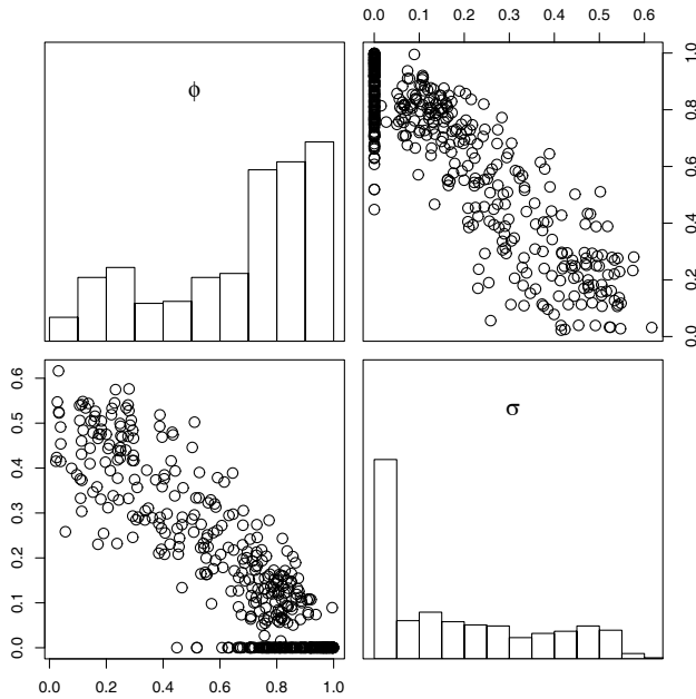
Fig. 6.10. Bootstrap distribution, B = 500 , of (i) the estimator of \phi (upper left), (ii) the estimator of \sigma_w (lower right), and (iii) the estimators jointly (off-diagonals). Only the values corresponding to \hat{\phi}^* \geq 0 are shown.
