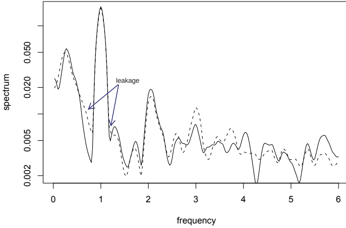
Fig. 4.11. Smoothed spectral estimates of the SOI without tapering (dashed line) and with full tapering (solid line); see Example 4.15 for details.
