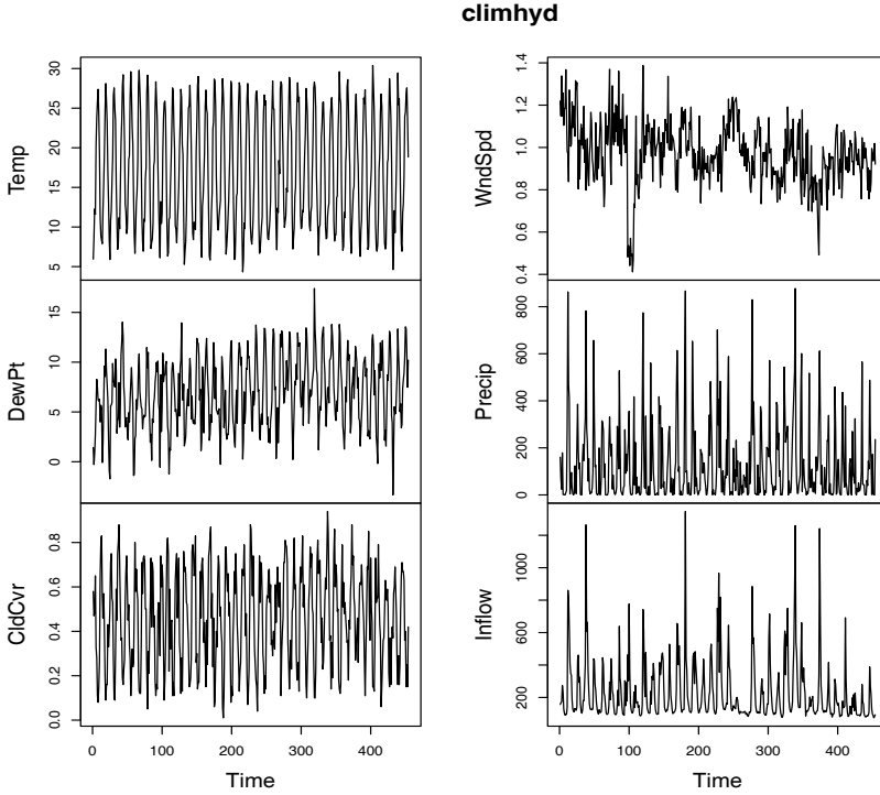
Fig. 7.3. Monthly values of weather and inflow at Lake Shasta.
