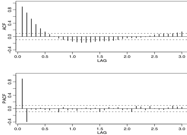
Fig. 5.11. ACF and PACF of the estimated noise \hat{\eta}_t departures from the transfer function model.
