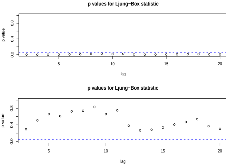
Fig. 3.20. Q-statistic p-values for the ARIMA(0, 1, 1) fit (top) and the ARIMA(1, 1, 1) fit (bottom) to the logged varve data.
