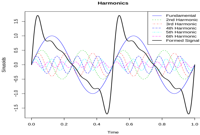
Fig. 4.8. A signal (thick solid line) formed by a fundamental sinusoid (thin solid line) oscillating at two cycles per unit time and its harmonics as specified in (4.57).
