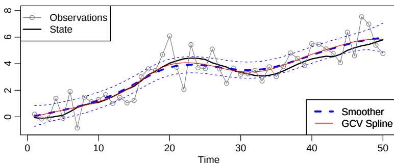
Fig. 6.6. Display for Example 6.10 : Simulated state process, \mu_t and observations y_t from the model (6.96) with n = 50 , \sigma_w = .1 and \sigma_v = 1 . Estimated smoother (dashed lines): \hat{\mu}_{t|n} and corresponding 95% confidence band. Gcv smoothing spline (thin solid line).
