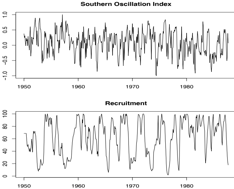
Fig. 1.5. Monthly SOI and Recruitment (estimated new fish), 1950-1987.
