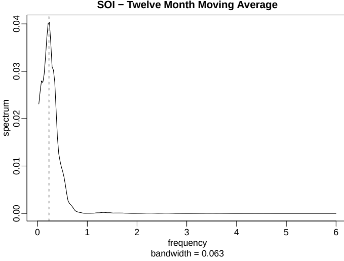
Fig. 4.16. Spectral analysis of SOI after applying a 12-month moving average filter. The vertical line corresponds to the 52-month cycle.
