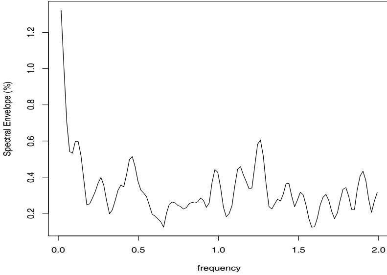
Fig. 7.26. Spectral envelope with respect to \mathcal{G} = \{x, |x|, x^2\} of the residuals from an MA(2) fit to the U.S. GNP growth rate data.
