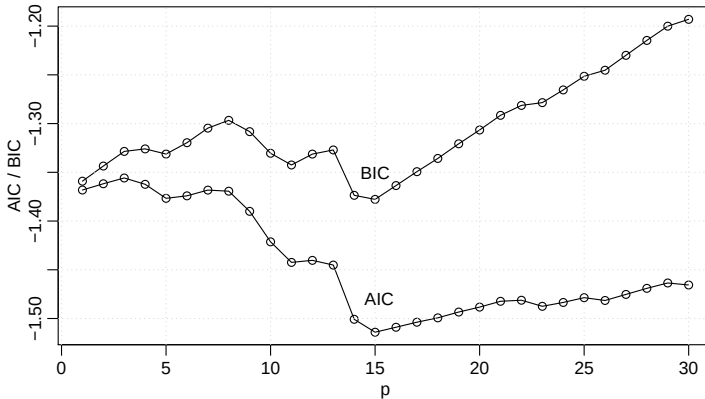
Fig. 4.12. Model selection criteria AIC and BIC as a function of order p for autoregressive models fitted to the SOI series.
