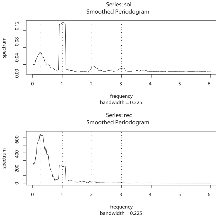
Fig. 4.6. The averaged periodogram of the SOI and Recruitment series n = 453 , n' = 480 , L = 9 , df = 17 , showing common peaks at the four year period, \omega = \frac{1}{4}\Delta = 1/48 cycles/month, the yearly period, \omega = 1\Delta = 1/12 cycles/month and some of its harmonics \omega = k\Delta for k = 2, 3 .
