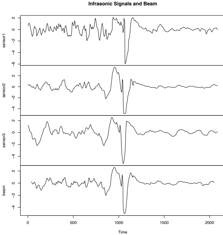
Fig. 7.6. Three series for a nuclear explosion detonated 25 km south of Christmas Island and the delayed average or beam. The time scale is 10 points per second.
