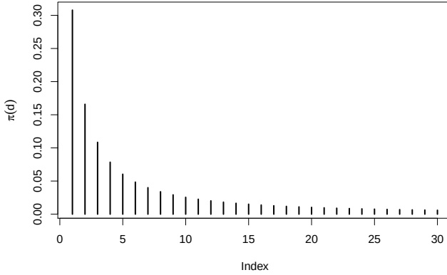
Fig. 5.2. Coefficients \pi_j(.384) , j = 1, 2, \dots, 30 in the representation (5.7).
