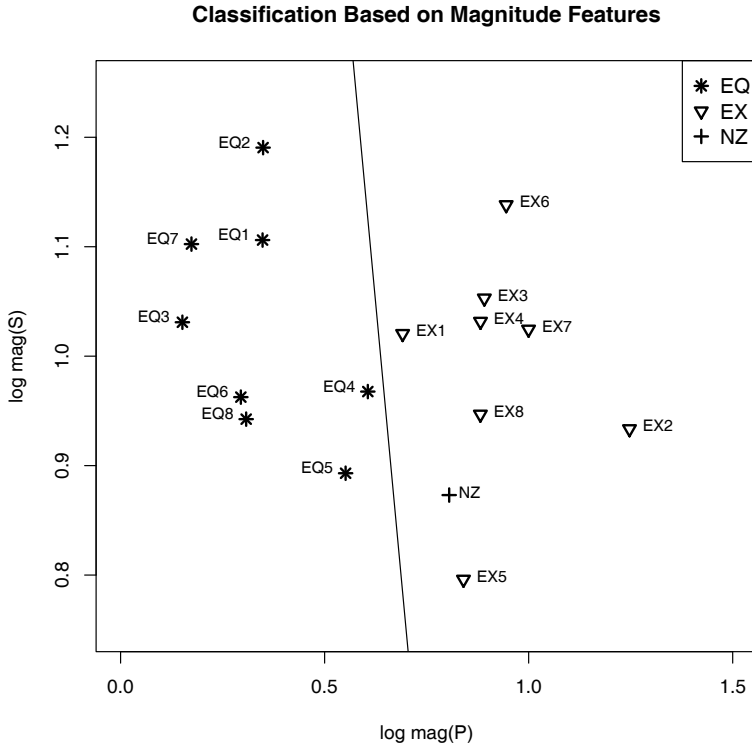
Fig. 7.13. Classification of earthquakes and explosions based on linear discriminant analysis using the magnitude features.
