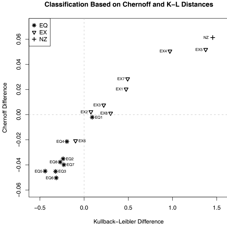
Fig. 7.15. Classification (by quadrant) of earthquakes and explosions using the Chernoff and Kullback-Leibler differences.
