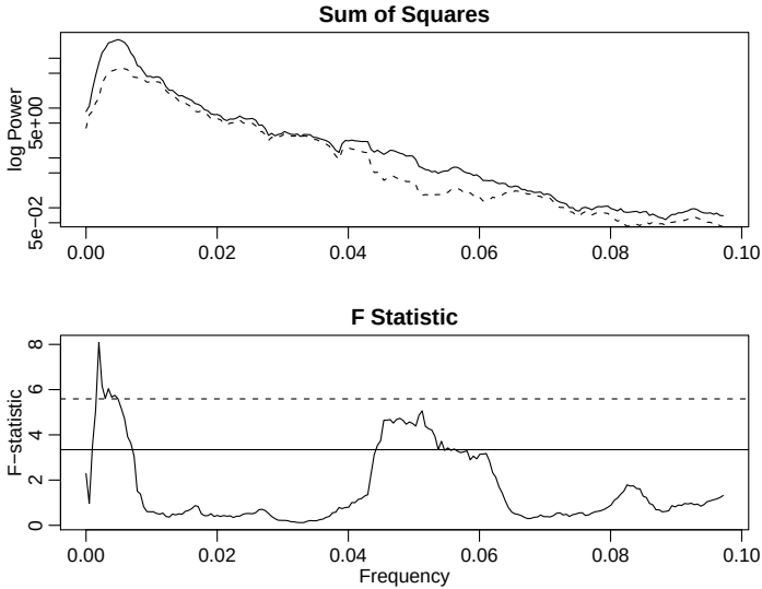
Fig. 7.7. Analysis of power for infrasound array on a log scale (top panel) with SST(\omega) shown as a solid line and SSE(\omega) as a dashed line. The F -statistics (bottom panel) showing detections with the dashed line based on an FDR level of .001 and the solid line corresponding null F quantile.
