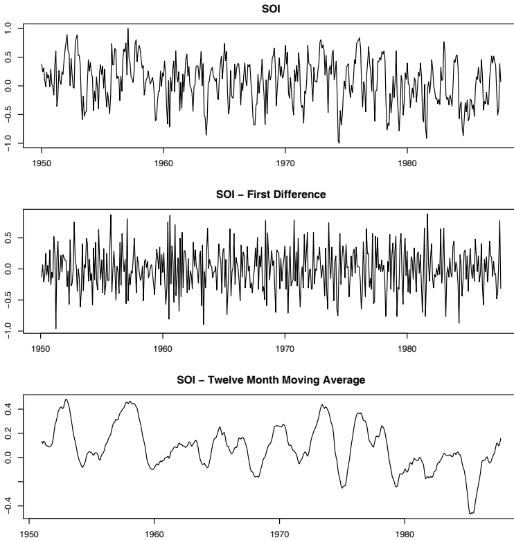
Fig. 4.15. SOI series (top) compared with the differenced SOI (middle) and a centered 12-month moving average (bottom).
