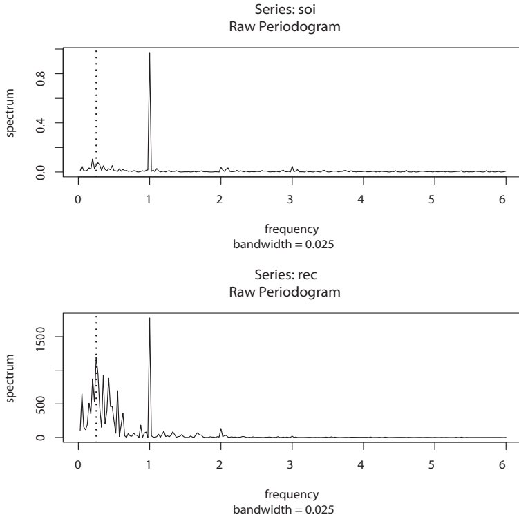
Fig. 4.5. Periodogram of SOI and Recruitment, n = 453 ( n' = 480 ), where the frequency axis is labeled in multiples of \Delta = 1/12 . Note the common peaks at \omega = 1\Delta = 1/12 , or one cycle per year (12 months), and \omega = \frac{1}{4}\Delta = 1/48 , or one cycle every four years (48 months).
