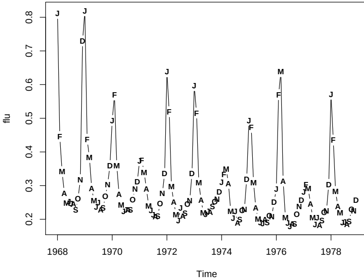
Fig. 5.7. U.S. monthly pneumonia and influenza deaths per 10,000.
