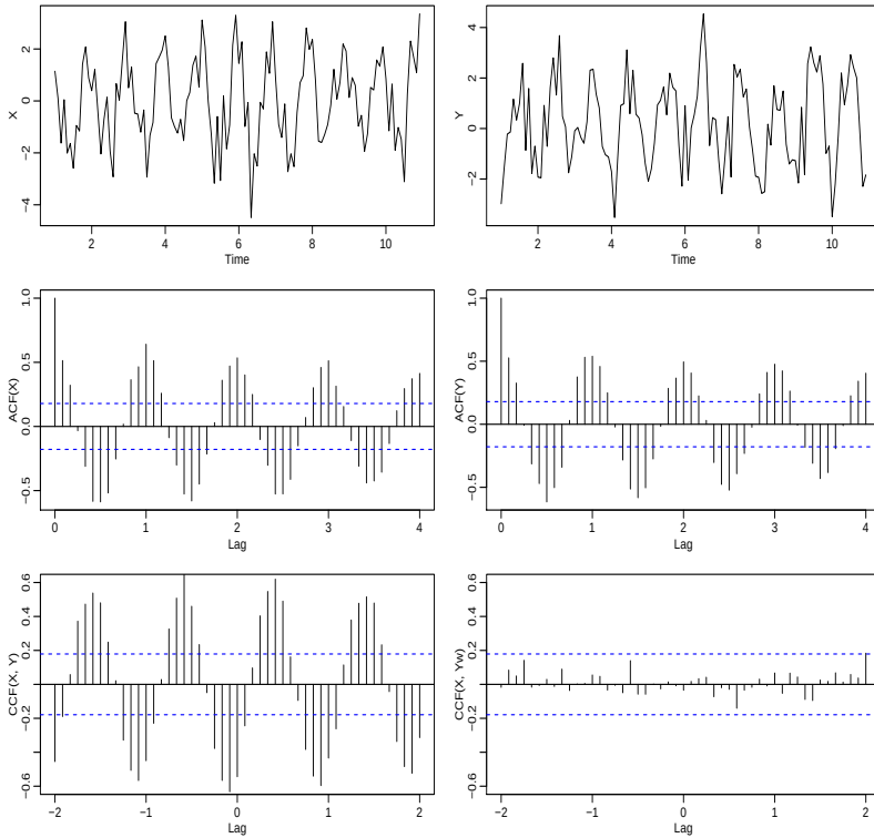
Fig. 1.16. Display for Example 1.27
