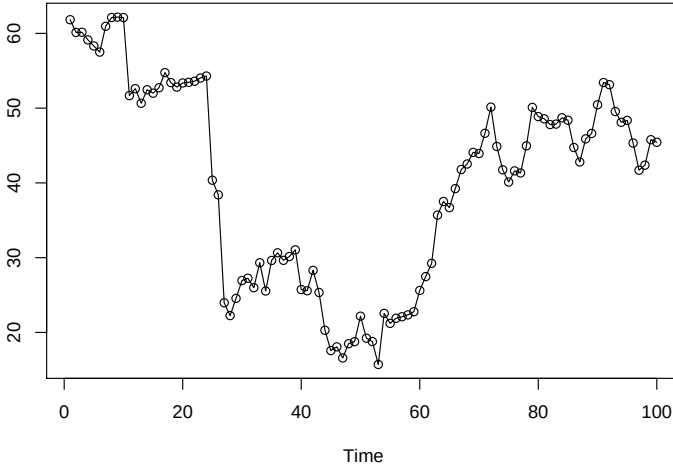
Fig. 3.11. One hundred observations generated from the model in Example 3.35 .
