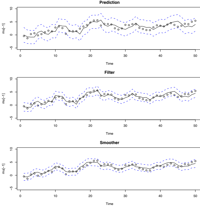
Fig. 6.3. Displays for Example 6.5 . The simulated values of \mu_t , for t = 1, \dots, 50 , given by (6.54) are shown as points. Top: The predictions \mu_t^{t-1} obtained via the Kalman filter are shown as a line. Error bounds, \mu_t^{t-1} \pm 2\sqrt{P_t^{t-1}} , are shown as dashed lines. Middle: The filter \mu_t^t obtained via the Kalman filter are shown as a line. Error bounds, \mu_t^t \pm 2\sqrt{P_t^t} , are shown as dashed lines. Bottom: The smoothers \mu_t^n obtained via the Kalman smoother are shown as a line. Error bounds, \mu_t^n \pm 2\sqrt{P_t^n} , are shown as dashed lines.
