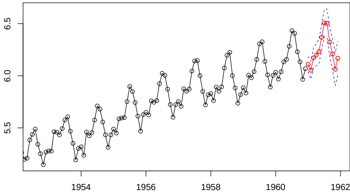
Fig. 3.28. Twelve month forecast using the \text{ARIMA}(0, 1, 1) \times (0, 1, 1)_{12} model on the logged air passenger data set.
