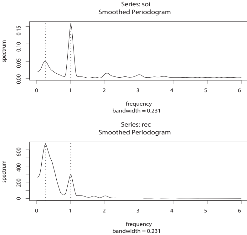
Fig. 4.9. Smoothed spectral estimates of the SOI and Recruitment series; see Example 4.14 for details.
