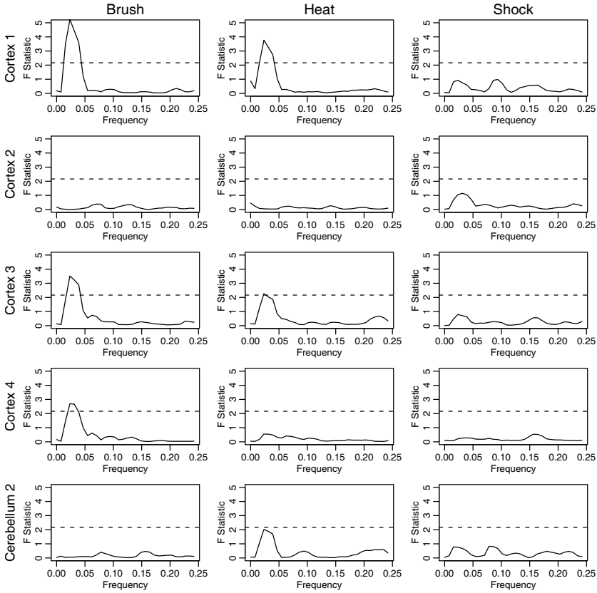
Fig. 7.11. Power in simultaneous linear compounds at five locations, enhancing brush, heat, and shock effects, L = 3 , F_{.001}(36, 120) = 2.16 .
