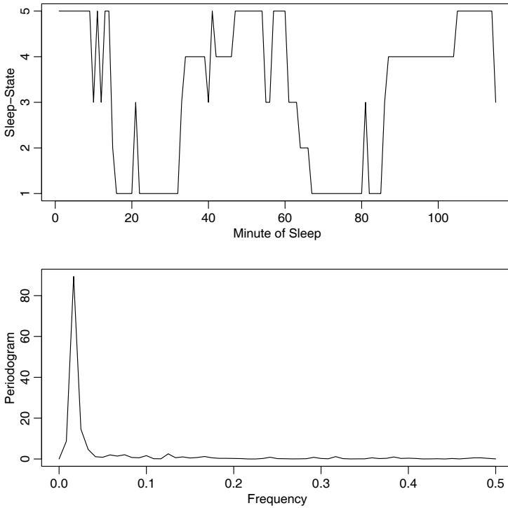
Fig. 7.23. [Top] Time plot of the EEG sleep state data in Table 7.7 using the scaling in (7.179). [Bottom] Periodogram of the EEG sleep state data in Figure 7.23 based on the scaling in (7.179). The peak corresponds to a frequency of approximately one cycle every 60 minutes.
