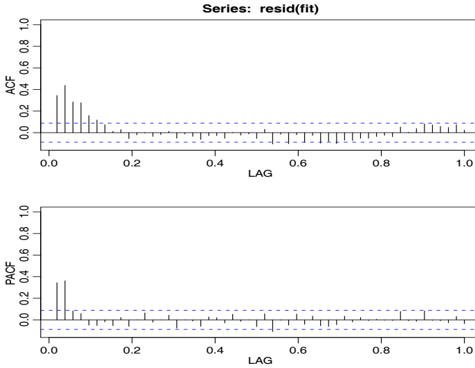
Fig. 3.22. Sample ACF and PACF of the mortality residuals indicating an AR(2) process.
