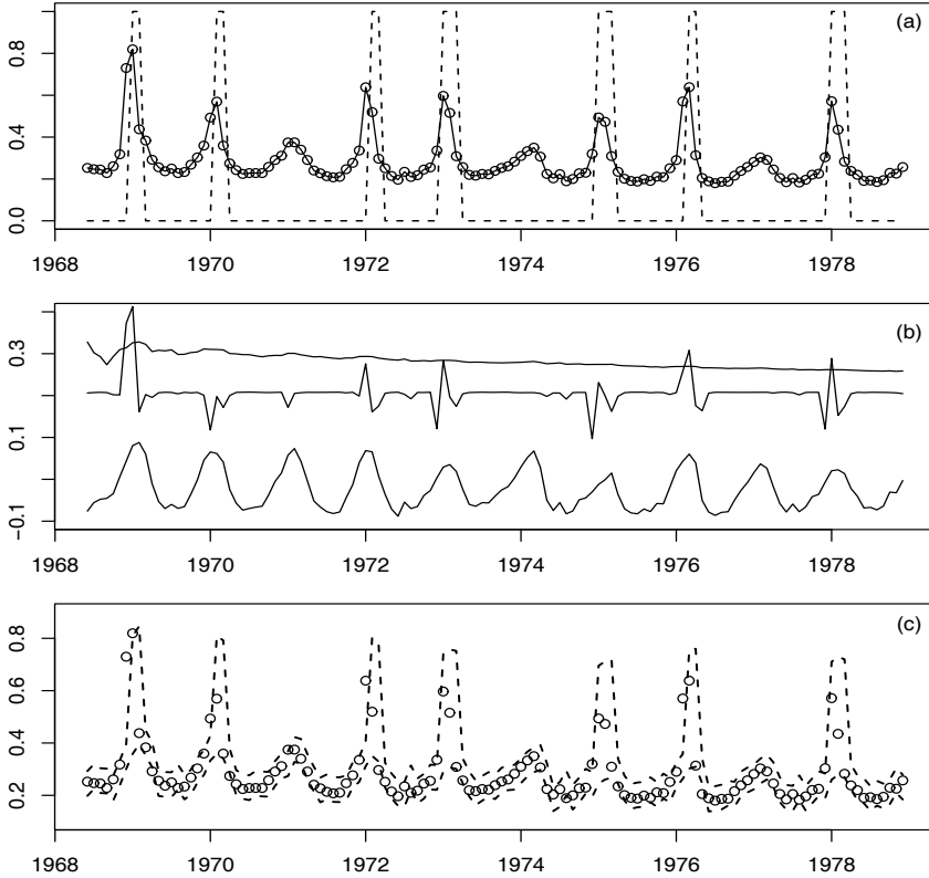
Fig. 6.11. (a) Influenza data, y_t , (line–points) and a prediction indicator (0 or 1) that an epidemic occurs in month t given the data up to month t - 1 (dashed line). (b) The three filtered structural components of influenza mortality: \hat{x}_{t1}^t (cyclic trace), \hat{x}_{t2}^t (spiked trace), and \hat{x}_{t3}^t (negative linear trace). (c) One-month-ahead predictions shown as upper and lower limits \hat{y}_t^{t-1} \pm 2\sqrt{\hat{P}_t^{t-1}} (dashed lines), of the number of pneumonia and influenza deaths, and y_t (points).
