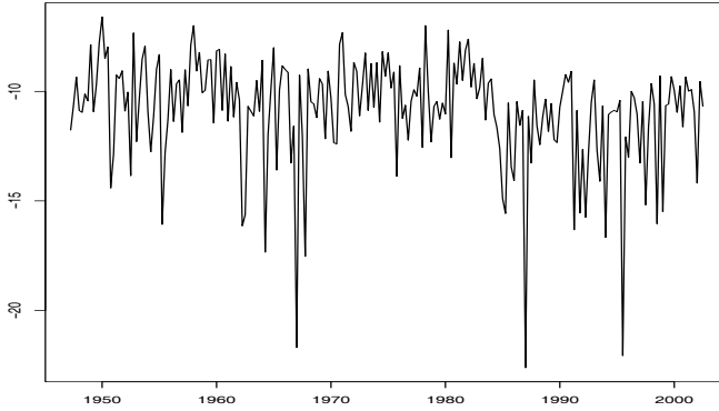
Fig. 6.14. Log of the squared residuals from an MA(2) fit on GNP growth rate.
