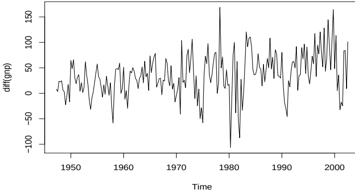
Fig. 3.16. First difference of the U.S. GNP data.
