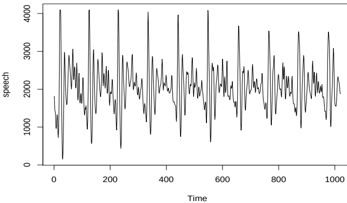
Fig. 1.3. Speech recording of the syllable aaa . . . hhh sampled at 10,000 points per second with n = 1020 points.
