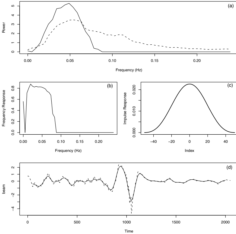
Fig. 7.8. (a) Estimated signal (solid line) and noise (dashed line) spectra; (b) Estimated frequency and (c) corresponding impulse filter responses; (d) Raw beam (dashed line) with superimposed filtered beam (solid line).
