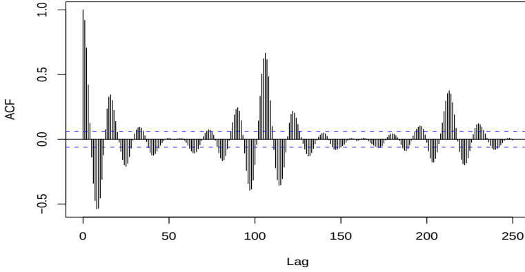
Fig. 1.14. ACF of the speech series.
