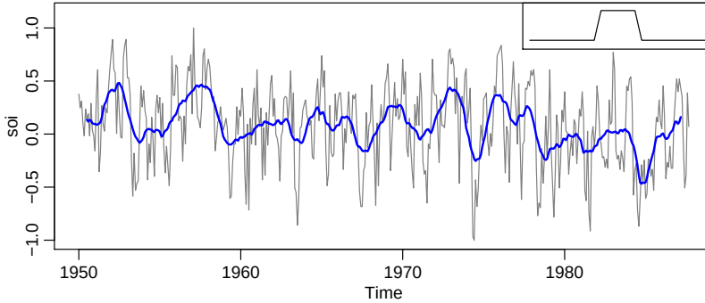
Fig. 2.12. Moving average smoother of SOI. The insert shows the shape of the moving average (“boxcar”) kernel [not drawn to scale] described in (2.49).
