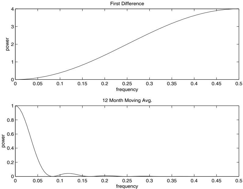
Fig. 4.17. Squared frequency response functions of the first difference and 12-month moving average filters.
