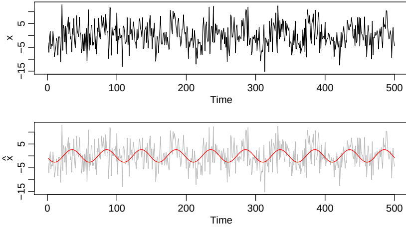
Fig. 2.10. Data generated by (2.35) [top] and the fitted line, (2.37), superimposed on the data [bottom].
