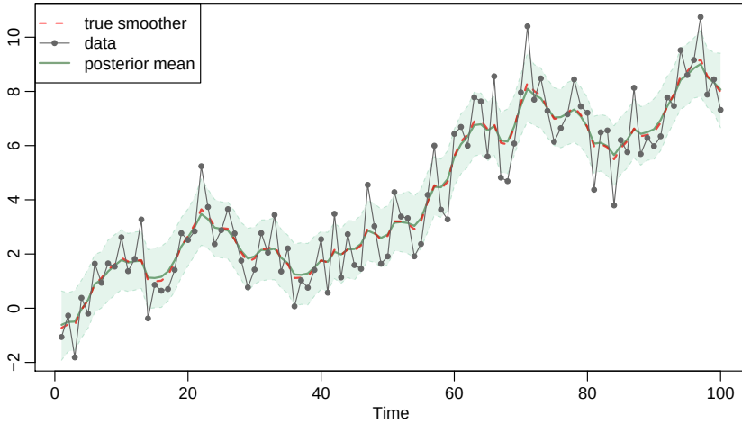
Fig. 6.17. Display for Example 6.22 : True smoother, x_t^n , the data y_t , and the posterior mean of the sampled smoother values; the filled in area shows 2.5% to 97.5%-tiles of the draws.
