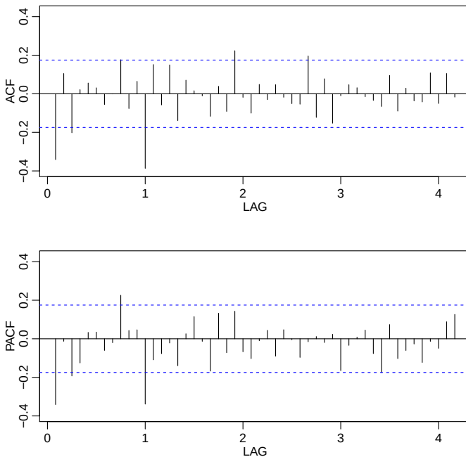
Fig. 3.26. Sample ACF and PACF of ddl x ( \nabla_{12} \nabla \log x_t ).
