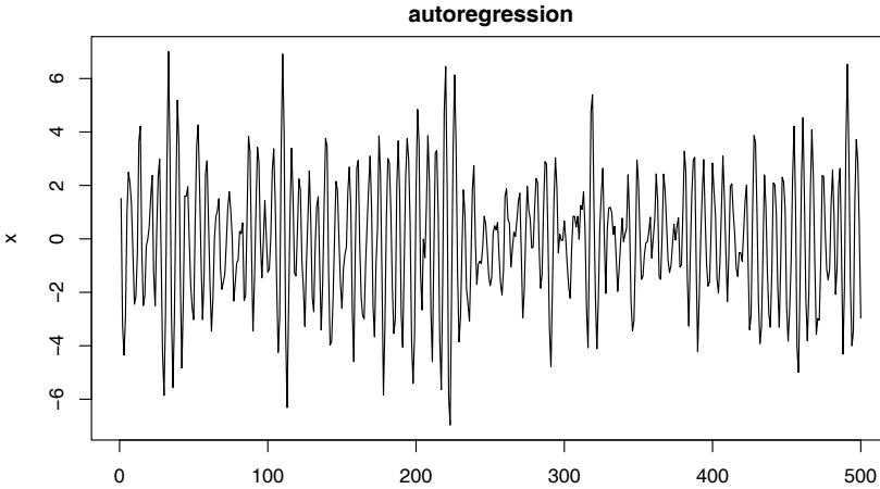
Fig. 1.9. Autoregressive series generated from model (1.2).
