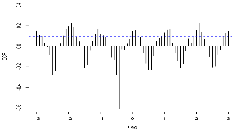
Fig. 5.10. Sample CCF of the prewhitened, detrended SOI and the similarly transformed Recruitment series; negative lags indicate that SOI leads Recruitment.
