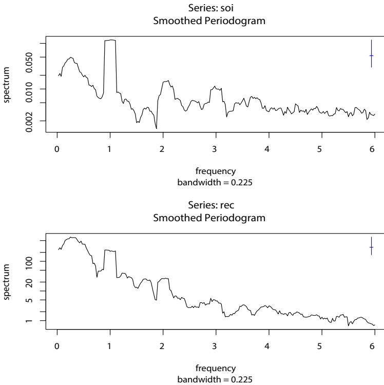
Fig. 4.7. Figure 4.6 with the average periodogram ordinates plotted on a \log_{10} scale. The display in the upper right-hand corner represents a generic 95% confidence interval.
