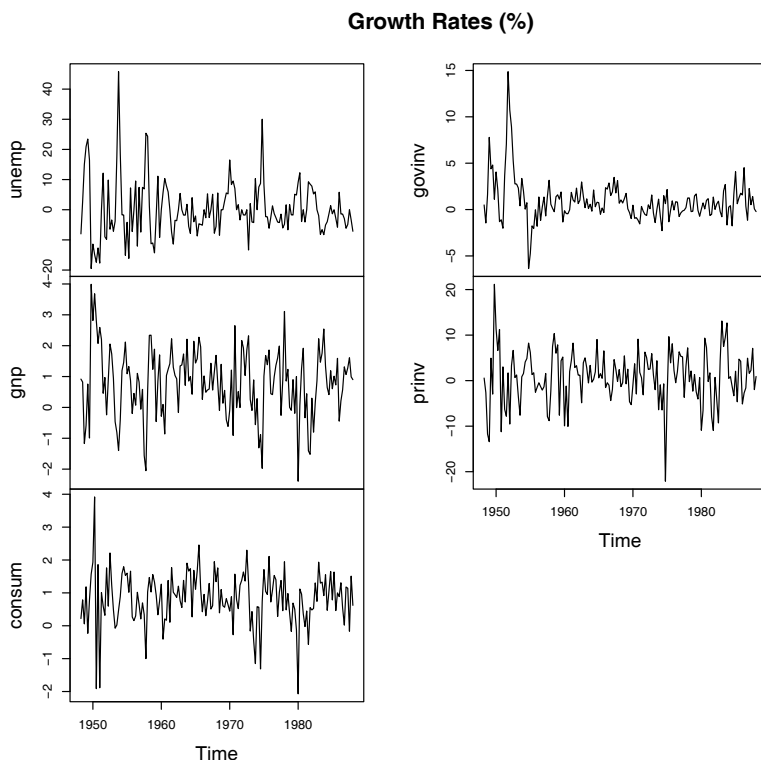
Fig. 7.19. The seasonally adjusted, quarterly growth rate (as percentages) of five macroeconomic series, unemployment, GNP, consumption, government investment, and private investment in the United States between 1948 and 1988, n = 160 values.
