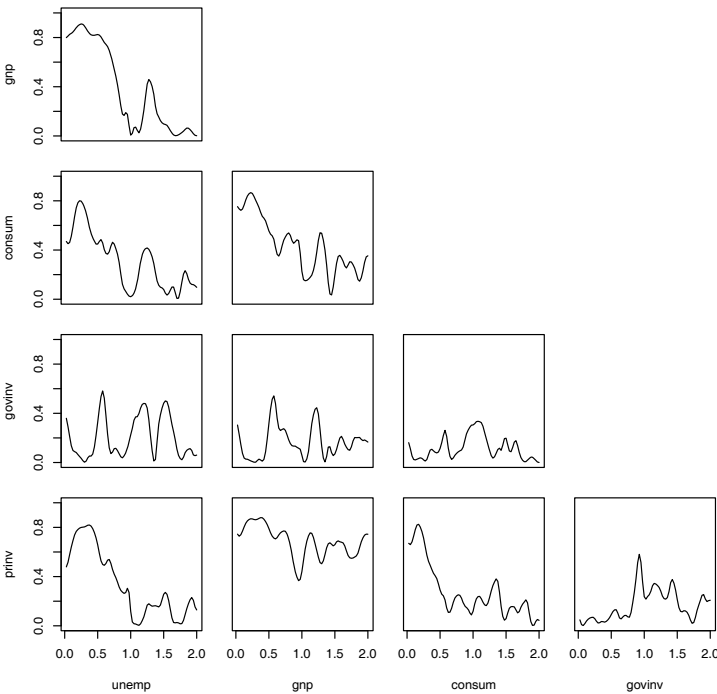
Fig. 7.21. The squared coherencies between the various series displayed in Figure 7.19.
