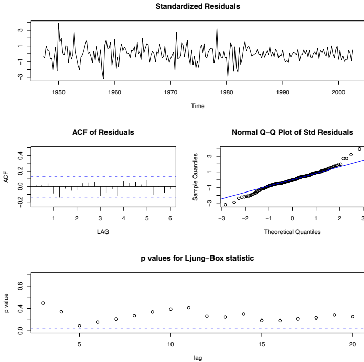
Fig. 3.19. Diagnostics of the residuals from MA(2) fit on GNP growth rate.
