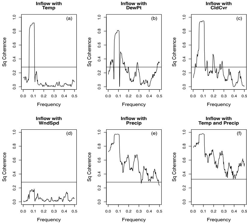
Fig. 7.4. Squared coherency between Lake Shasta inflow and (a) temperature; (b) dew point; (c) cloud cover; (d) wind speed; (e) precipitation. The multiple coherency between inflow and temperature – precipitation jointly is displayed in (f). In each case, the .001 threshold is exhibited as a horizontal line.
