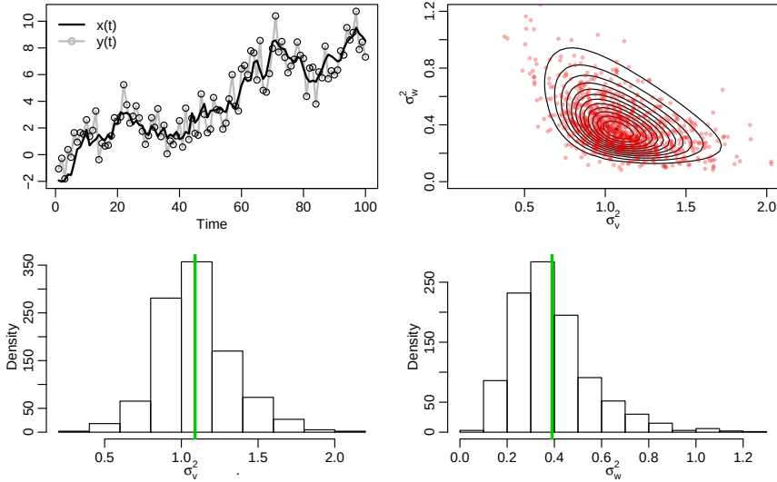
Fig. 6.16. Display for Example 6.22 : Top: Generated states, x_t and data y_t . Contours of the likelihood (solid line) of the data and sampled posterior values as points. Bottom: Marginal sampled posteriors and posterior means (vertical lines) of each variance component. The true values are \sigma_v^2 = 1 and \sigma_w^2 = .5 .
