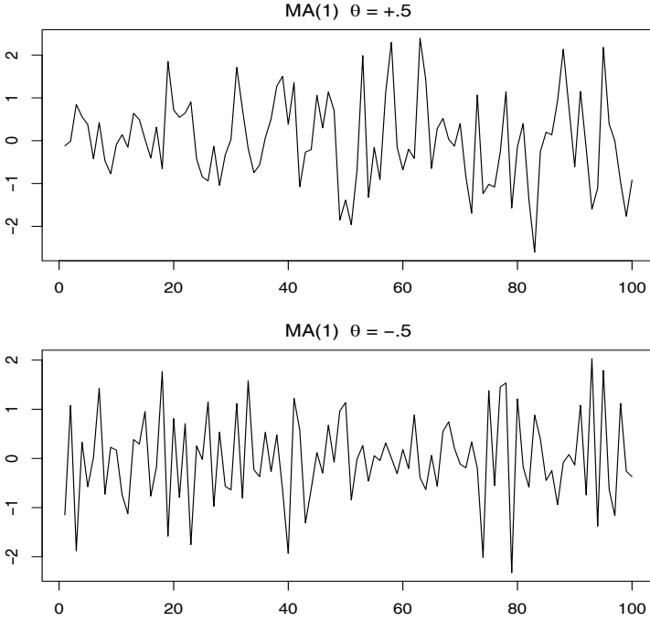
Fig. 3.2. Simulated MA(1) models: \theta = .5 (top); \theta = -.5 (bottom).
