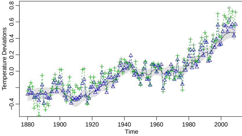
Fig. 6.4. Plot for Example 6.7 . The dashed lines are the two average global temperature deviations shown in Figure 6.2 . The solid line is the estimated smoother \hat{x}_t^n , and the corresponding two root mean square error bounds is the gray area.
