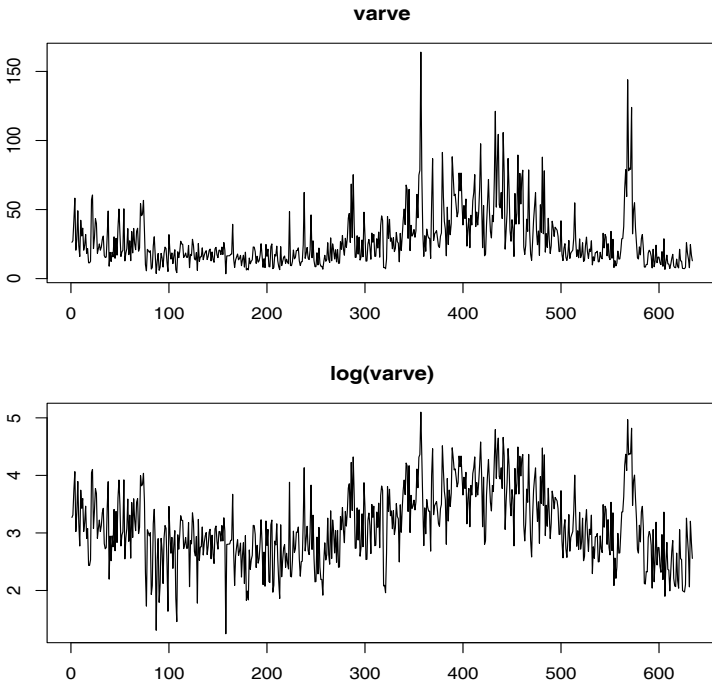
Fig. 2.6. Glacial varve thicknesses (top) from Massachusetts for n = 634 years compared with log transformed thicknesses (bottom).
