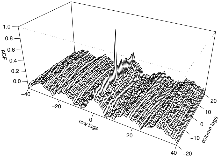
Fig. 1.19. Two-dimensional autocorrelation function for the soil temperature data.
