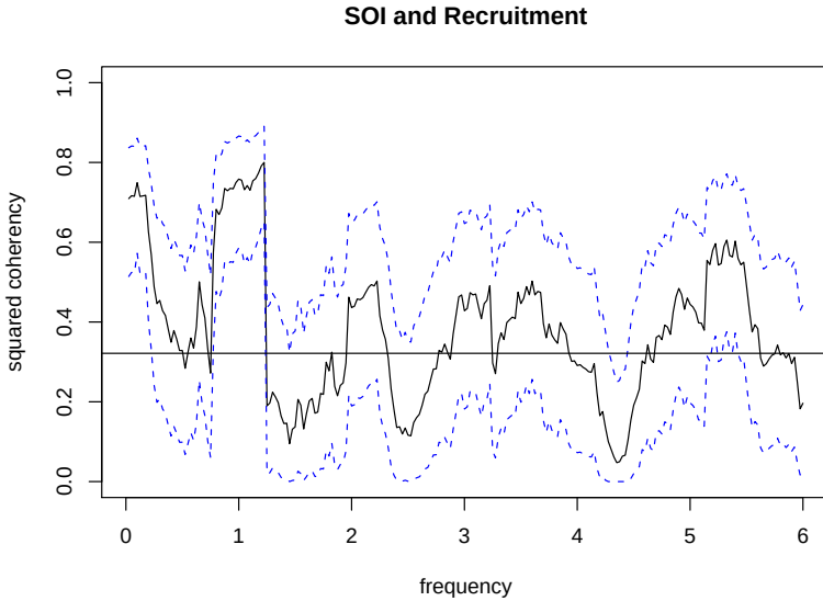
Fig. 4.14. Squared coherency between the SOI and Recruitment series; L = 19 , n = 453 , n' = 480 , and \alpha = .001 . The horizontal line is C_{.001} .
