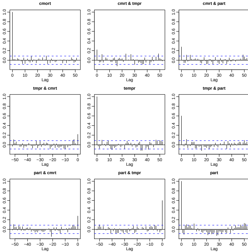
Fig. 5.12. ACFs (diagonals) and CCFs (off-diagonals) for the residuals of the three-dimensional VAR(2) fit to the LA mortality – pollution data set. On the off-diagonals, the second-named series is the one that leads.
