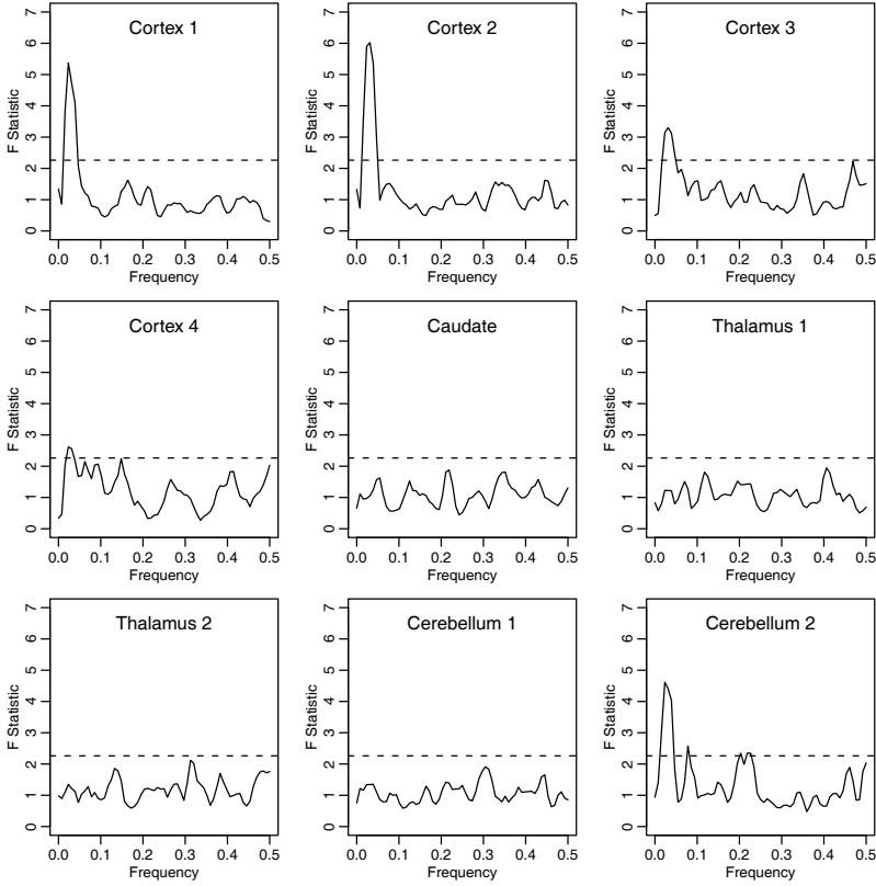
Fig. 7.9. Frequency-dependent equality of means tests for fMRI data at 9 brain locations. L = 3 and critical value F_{.001}(30, 120) = 2.26 .
