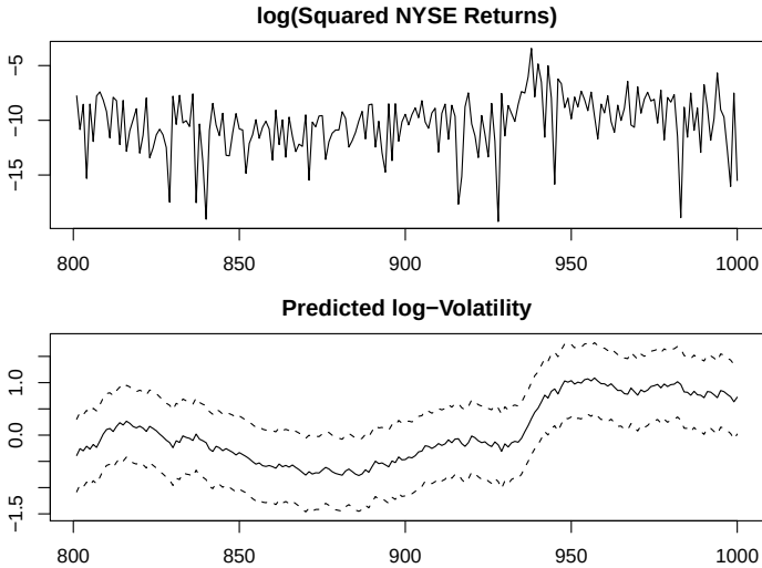
Fig. 6.12. Two hundred observations of y_t = \log r_t^2 , for 801 \leq t \leq 1000 , where r_t is the daily return of the NYSE (top); the crash of October 19, 1987 occurs at t = 938 . Corresponding one-step-ahead predicted log volatility, \log \sigma_t^2 , with \pm 2 standard prediction errors (bottom).
