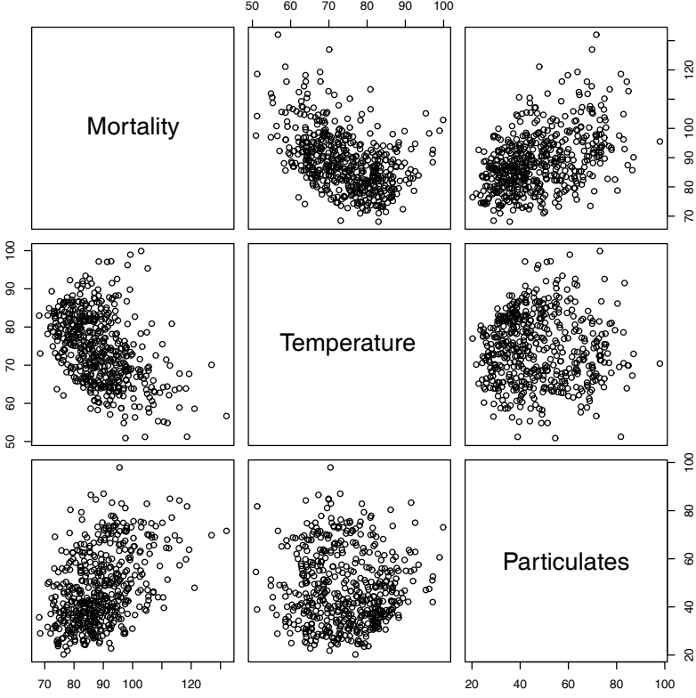
Fig. 2.3. Scatterplot matrix showing relations between mortality, temperature, and pollution.
