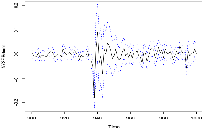
Fig. 5.6. GARCH predictions of the NYSE volatility, \pm 2\hat{\sigma}_t , displayed as dashed lines.
