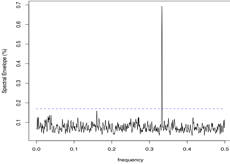
Fig. 7.24. Smoothed sample spectral envelope of the BNRF1 gene from the Epstein–Barr virus.
