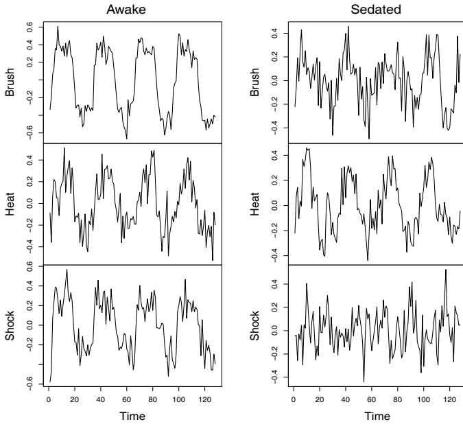
Fig. 7.1. Mean response of subjects to various combinations of periodic stimuli measured at the cortex (primary somatosensory, contralateral). In the first column, the subjects are awake, in the second column the subjects are under mild anesthesia. In the first row, the stimulus is a brush on the hand, the second row involves the application of heat, and the third row involves a low level shock.
