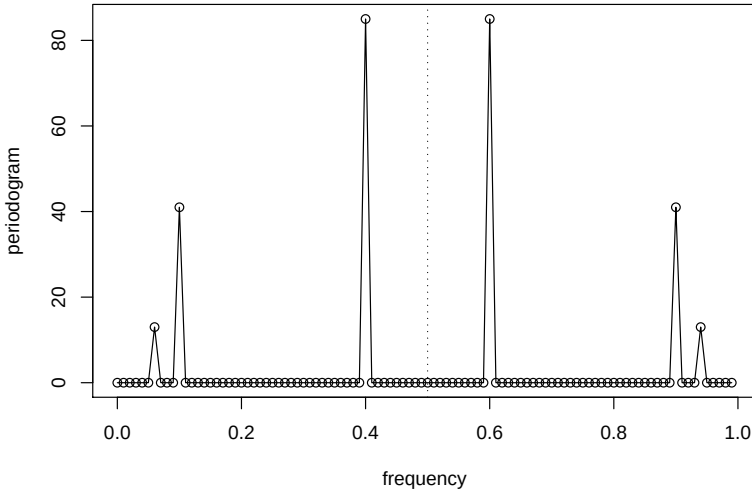
Fig. 4.2. Periodogram of the data generated in Example 4.1 .
