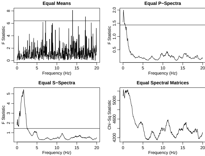
Fig. 7.12. Tests for equality of means, spectra, and spectral matrices for the earthquake and explosion data p = 2 , L = 21 , n = 1024 points at 40 points per second.
