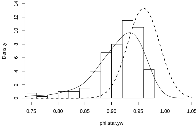
Fig. 3.13. Bootstrap histogram of \hat{\phi} based on 200 bootstraps; a density estimate based on the histogram (solid line) and the corresponding asymptotic normal density (dashed line).
