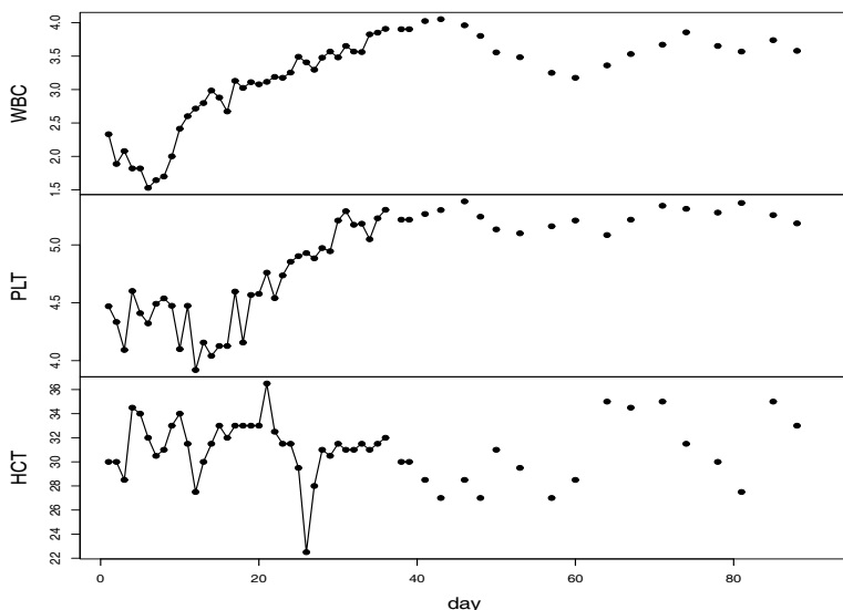
Fig. 6.1. Longitudinal series of blood parameter levels monitored, log (white blood count) [WBC; top], log (platelet) [PLT; middle], and hematocrit [HCT; bottom], after a bone marrow transplant ( n = 91 days).
