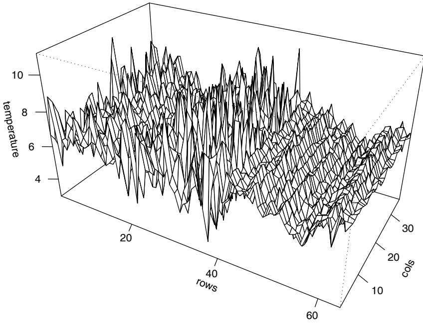
Fig. 1.17. Two-dimensional time series of temperature measurements taken on a rectangular field ( 64 \times 36 with 17-foot spacing). Data are from Bazza et al. (1988).
