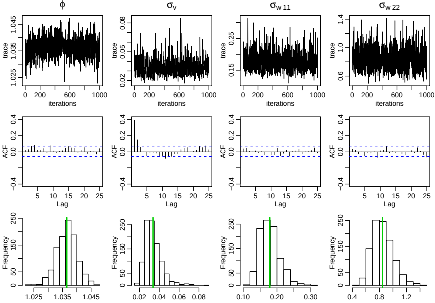
Fig. 6.18. Parameter estimation results for Example 6.23 . The top row displays the traces of 1000 draws after burn-in. The middle row displays the ACF of the traces. The sampled posteriors are displayed in the last row (the mean is marked by a solid vertical line).
