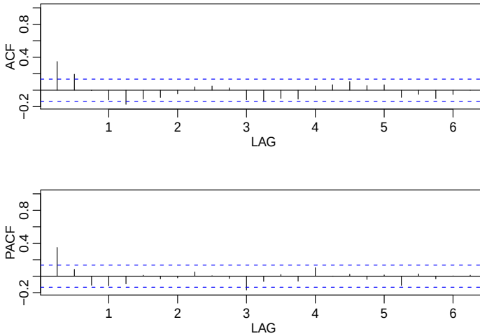
Fig. 3.18. Sample ACF and PACF of the GNP quarterly growth rate. Lag is in terms of years.
