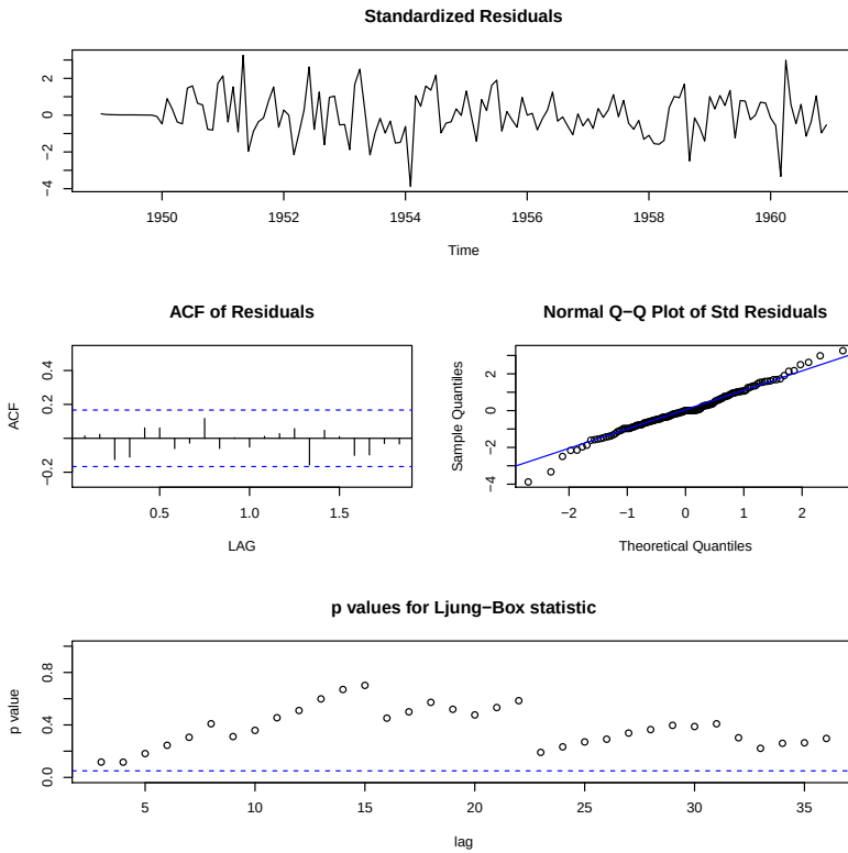
Fig. 3.27. Residual analysis for the \text{ARIMA}(0, 1, 1) \times (0, 1, 1)_{12} fit to the logged air passengers data set.
