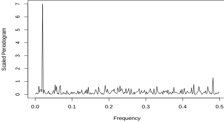
Fig. 2.11. The scaled periodogram, (2.42), of the 500 observations generated by (2.35); the data are displayed in Figure 1.11 and Figure 2.10.
