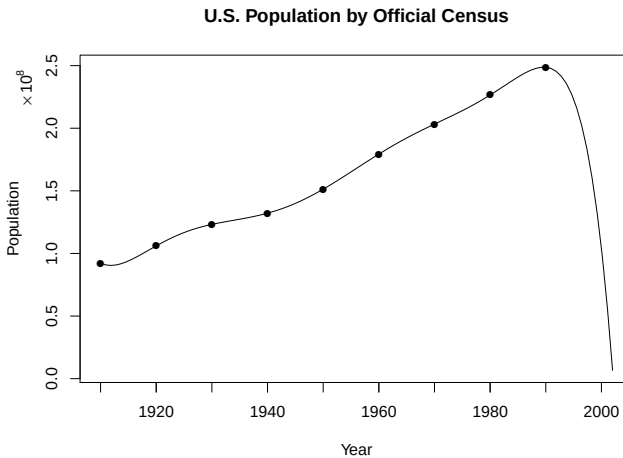
Fig. 3.21. A perfect fit and a terrible forecast.
