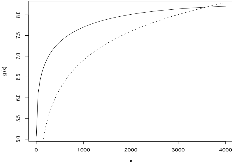
Fig. 7.30. The estimated optimal transformation at \omega_0 as given in (7.189) (solid line) and the log transformation, g(x) = \ln(x) (dashed line).
