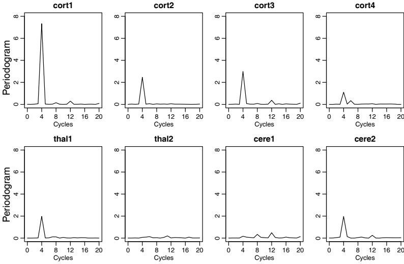
Fig. 7.17. The individual periodograms of x_{tk} , for k = 1, \dots, 8 , in Example 7.14 .
