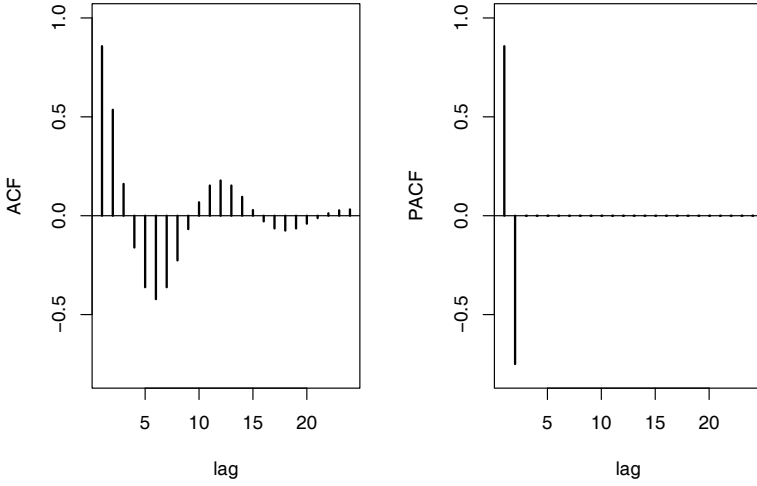
Fig. 3.5. The ACF and PACF of an AR(2) model with \phi_1 = 1.5 and \phi_2 = -.75 .
