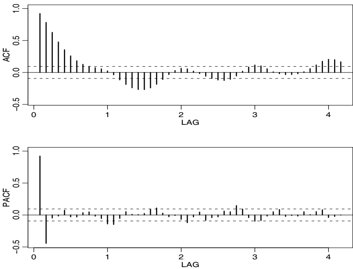
Fig. 3.6. ACF and PACF of the Recruitment series. Note that the lag axes are in terms of season (12 months in this case).
