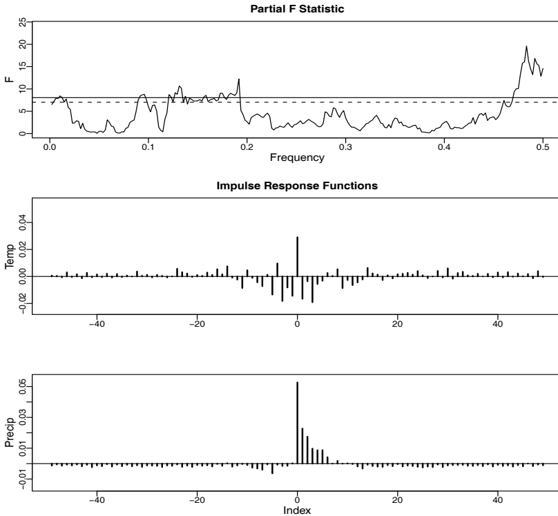
Fig. 7.5. Partial F -statistics [top] for testing whether temperature adds to the ability to predict Lake Shasta inflow when precipitation is included in the model. The dashed line indicates the .001 FDR level and the solid line represents the corresponding quantile of the null F distribution. Multiple impulse response functions for the regression relations of temperature [middle] and precipitation [bottom].
