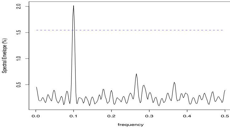
Fig. 7.29. Spectral envelope with respect to \mathcal{G} = \{x, \sqrt{x}, \sqrt[3]{x}\} of data generated from (7.188).
