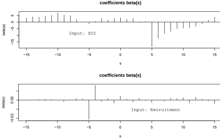
Fig. 4.18. Estimated impulse response functions relating SOI to Recruitment (top) and Recruitment to SOI (bottom) L = 15 , M = 32 .
