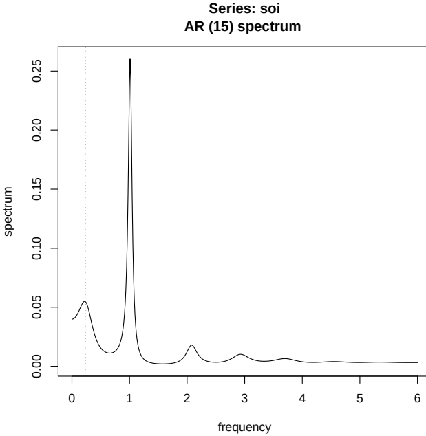
Fig. 4.13. Autoregressive spectral estimator for the SOI series using the AR(15) model selected by AIC, AICc, and BIC. The first peak (marked by a vertical dotted line) corresponds to the El Niño period of 52 months.
