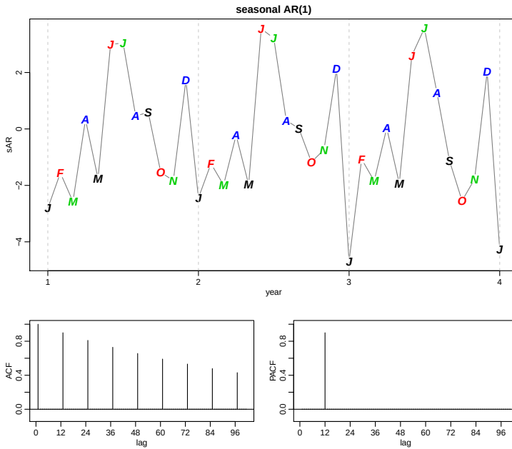
Fig. 3.23. Data generated from a seasonal ( s = 12 ) AR(1), and the true ACF and PACF of the model x_t = .9x_{t-12} + w_t .
