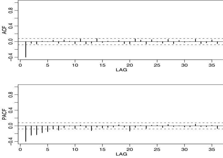
Fig. 3.9. ACF and PACF of transformed glacial varves.
