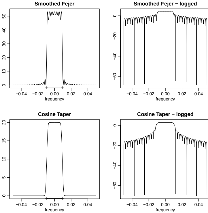
Fig. 4.10. Averaged Fejér window (top row) and the corresponding cosine taper window (bottom row) for L = 9 , n = 480 . The extra tic marks on the horizontal axis of the left-hand plots exhibit the predicted bandwidth, B_w = 9/480 = .01875 .
