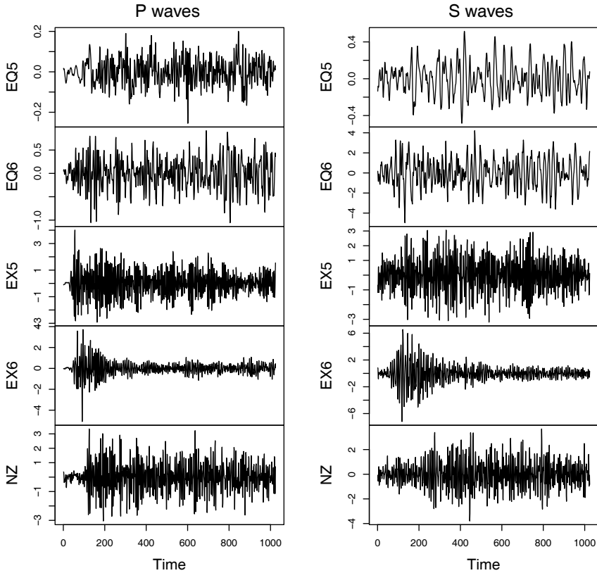
Fig. 7.2. Various bivariate earthquakes (EQ) and explosions (EX) recorded at 40 pts/sec compared with an event NZ (Novaya Zemlya) of unknown origin. Compressional waves, also known as primary or P waves, travel fastest in the Earth's crust and are first to arrive. Shear waves propagate more slowly through the Earth and arrive second, hence they are called secondary or S waves.
