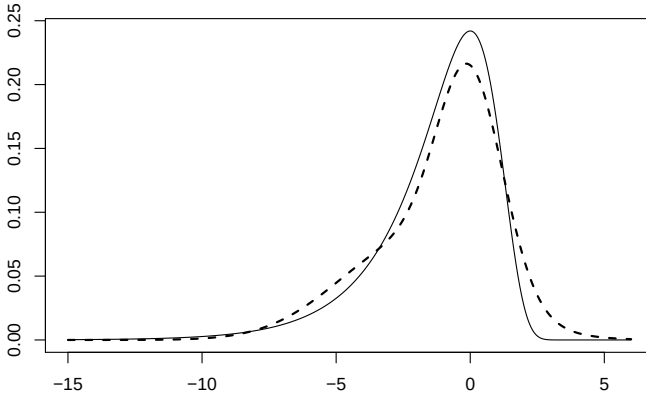
Fig. 6.13. Density of the log of a \chi_1^2 as given by (6.180) (solid line) and the fitted normal mixture (dashed line) from the NYSE example.
