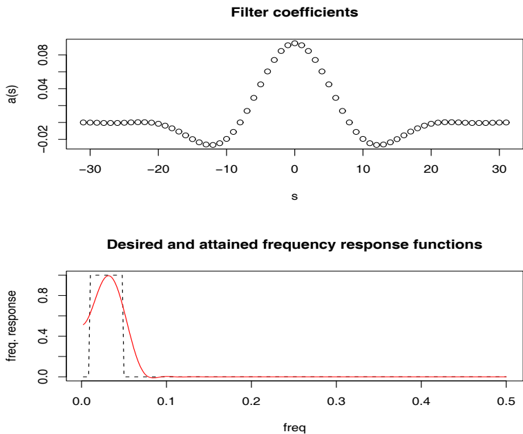
Fig. 4.19. Filter coefficients (top) and frequency response functions (bottom) for designed SOI filters.
