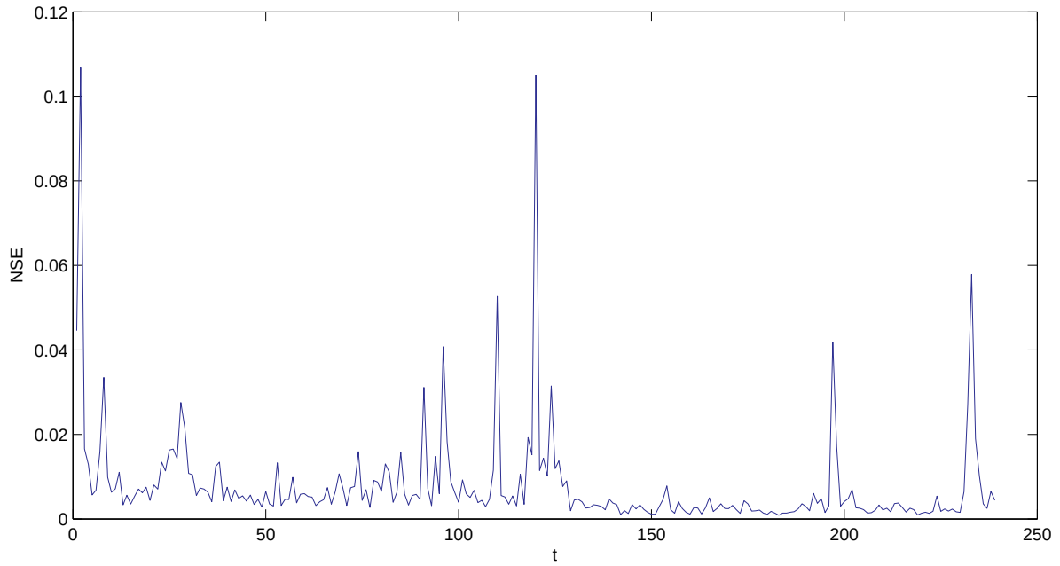
Figure 13: Numerical standard error of log predictive likelihoods \log p(y_t | y_{1:t-1}) . J = 16 , N = 4096 , D_1 = 0.5 , D_2 = 0.2 , R = 55 .
